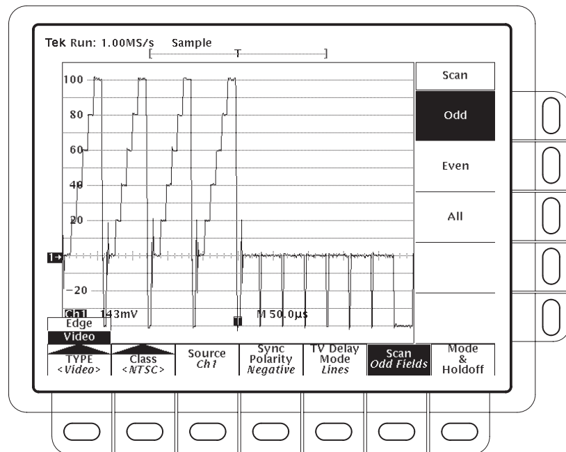
Figure 3-68: Main Trigger Menu — Video Type
