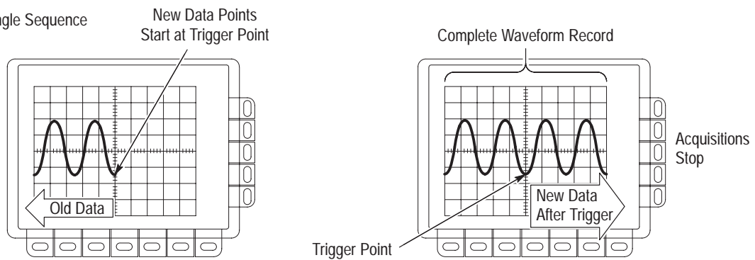
Figure 3-53: Roll Mode (500 Point Record Length)
