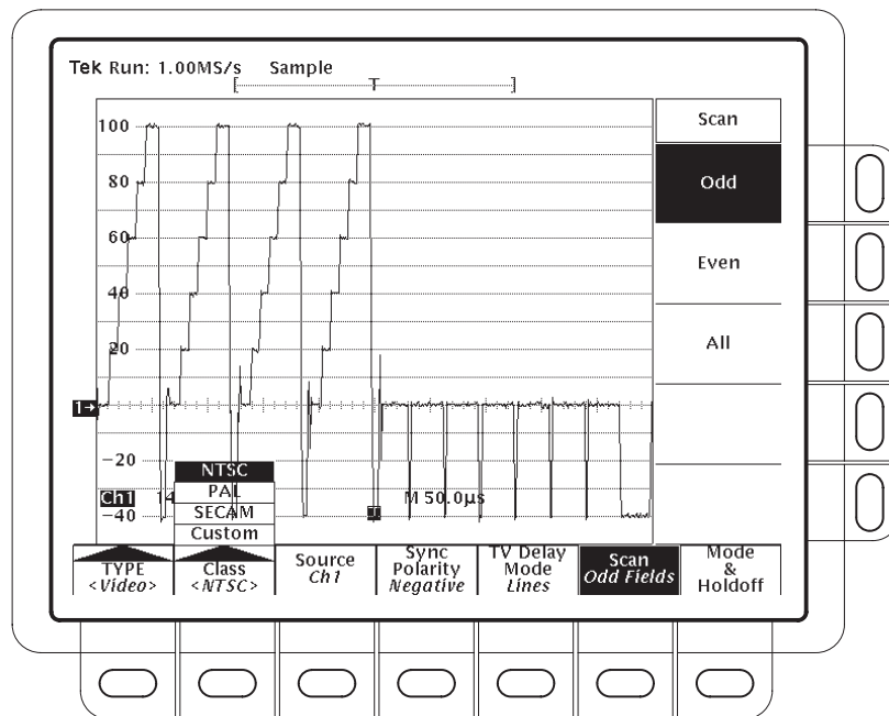
Figure 3-69: Video Trigger Menu — Class
