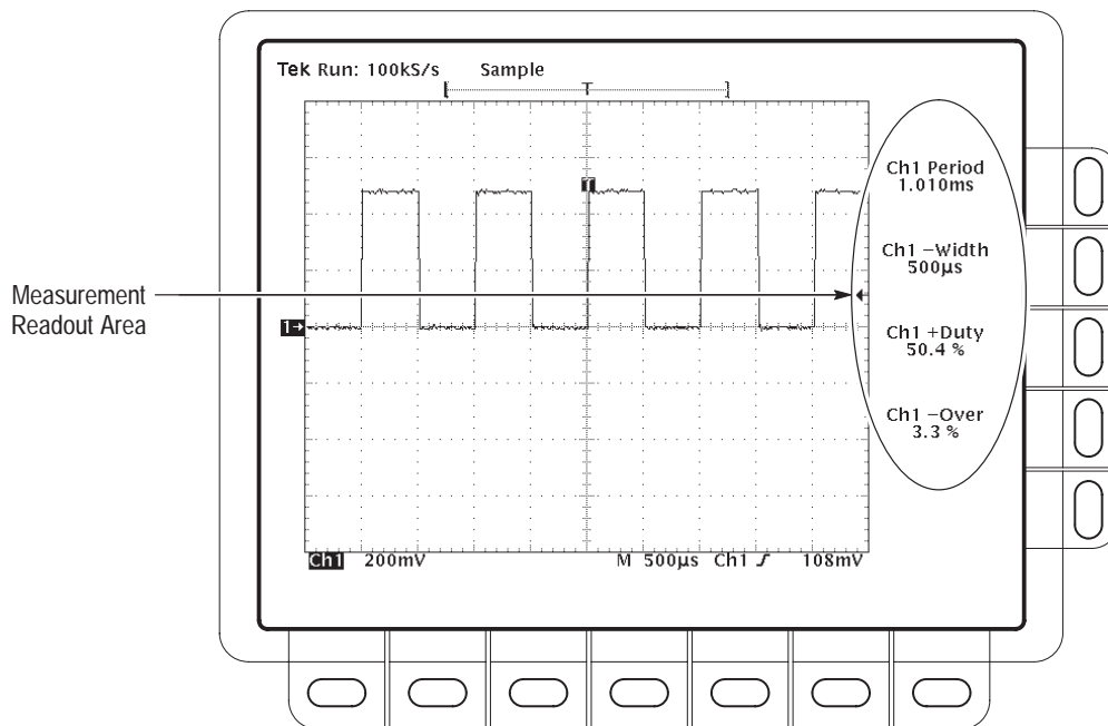
Figure 3-38: Measurement Readouts
