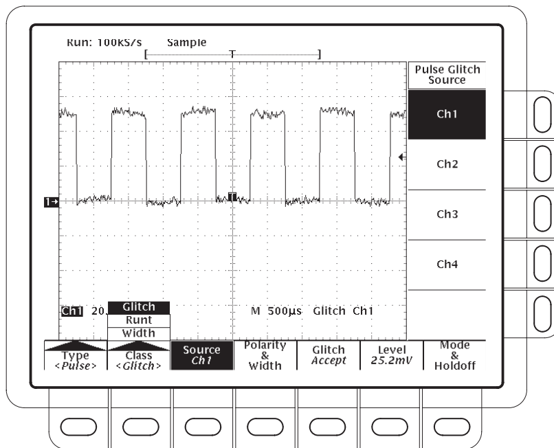
Figure 3-49: Main Trigger Menu — Glitch Class
