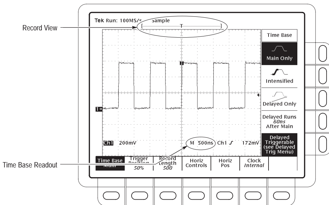
Figure 3-30: Record View and Time Base Readouts
