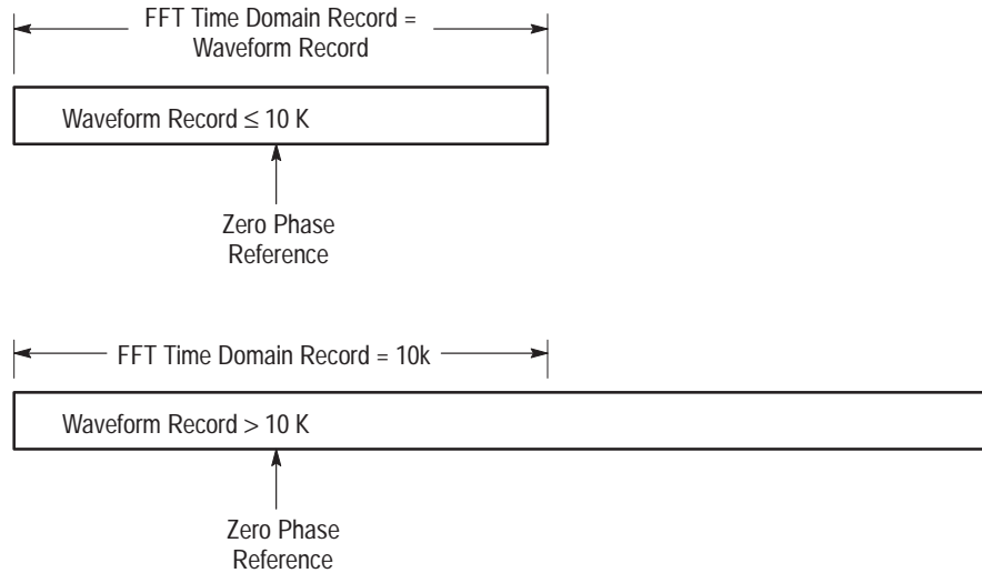
Figure 3-19: Waveform Record vs. FFT Time Domain Record
