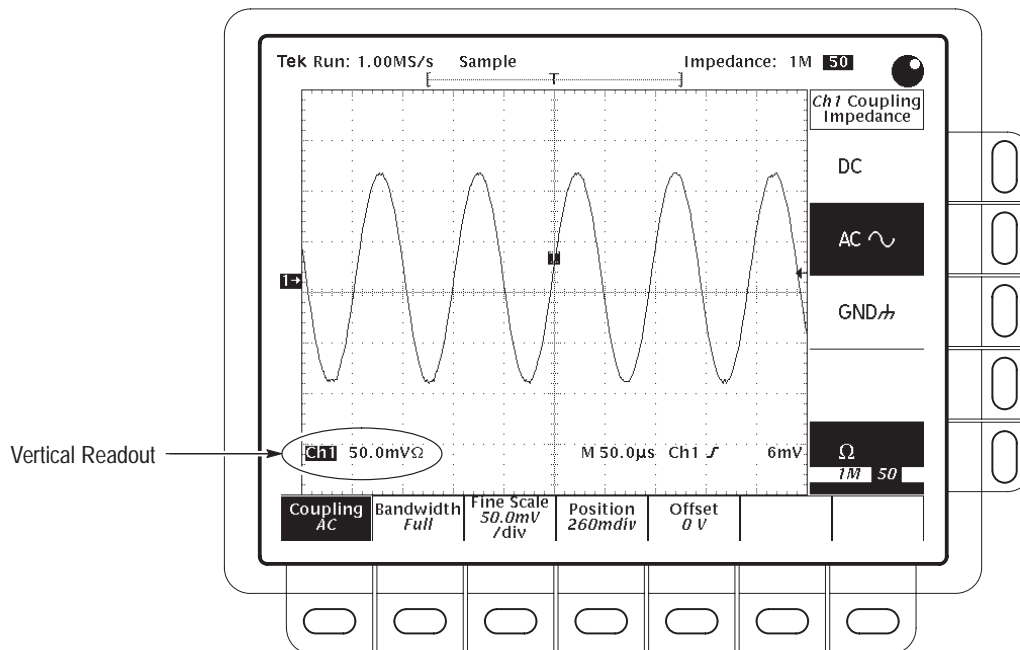
Figure 3-67: Vertical Readouts and Channel Menu
