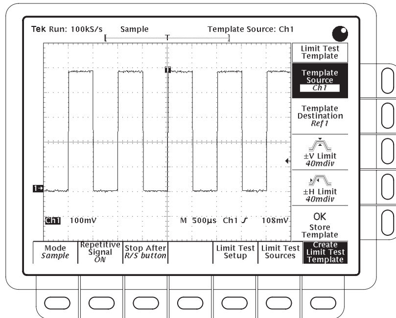
Figure 3-34: Acquire Menu — Create Limit Test Template
