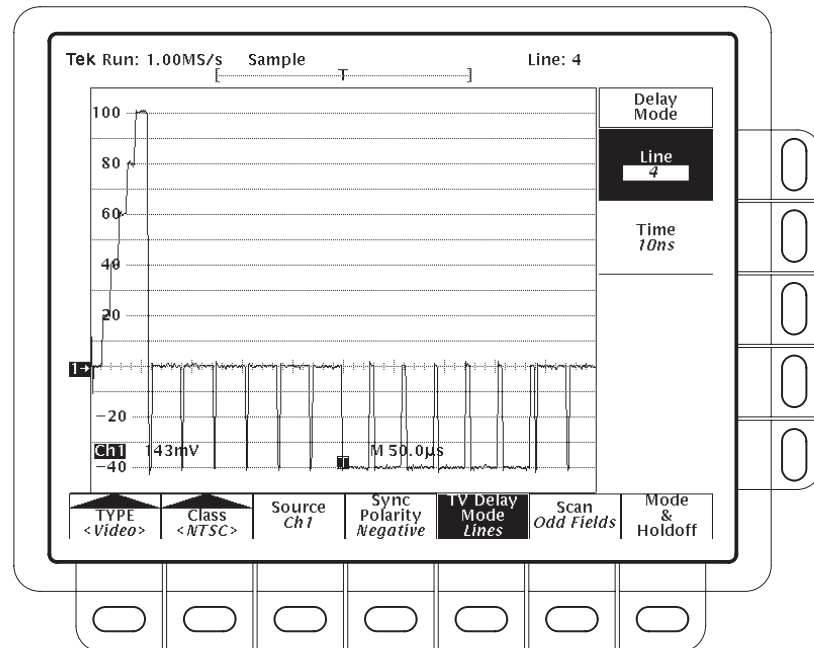
Figure 3-70: Video Trigger Menu — TV Delay Mode
