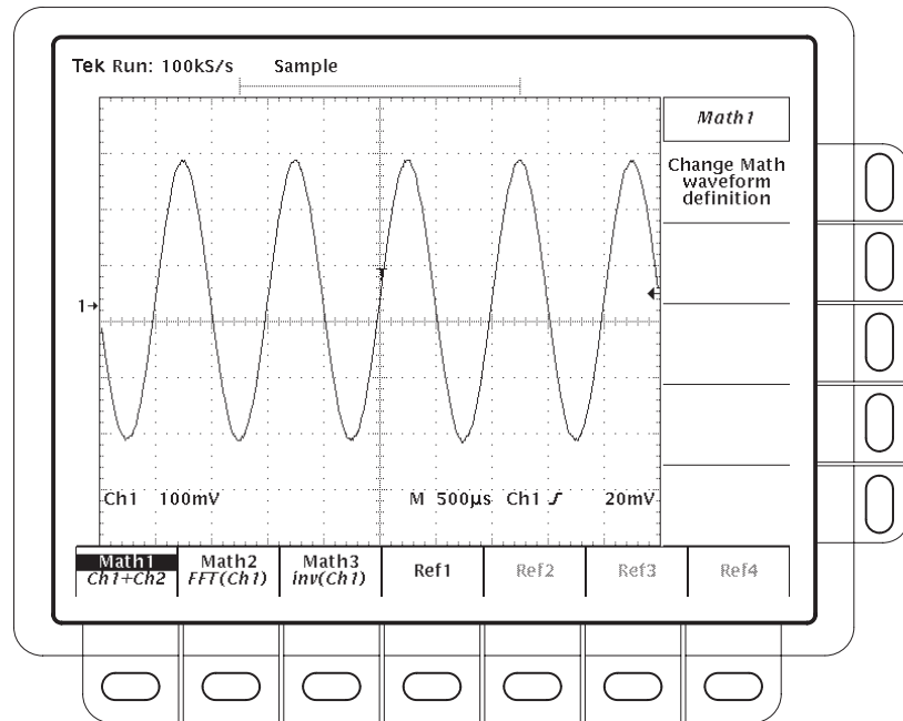
Figure 3-57: More Menu
