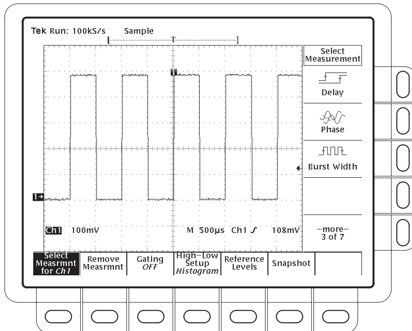
Figure 3-39: Measure Menu
