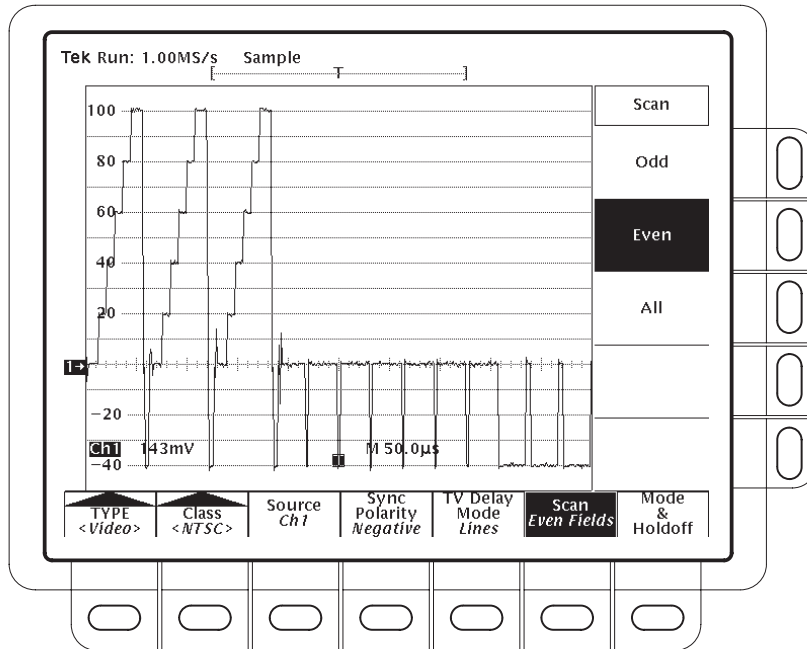
Figure 3-71: Video Trigger — Scan Parameter
