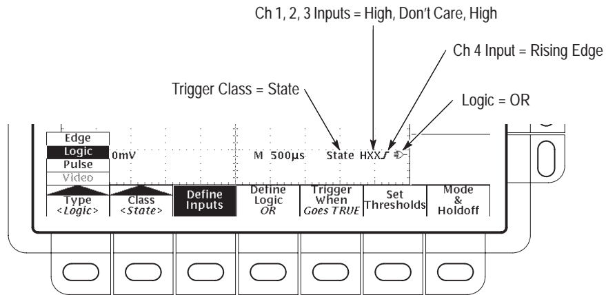
Figure 3-35: Logic Trigger Readouts
