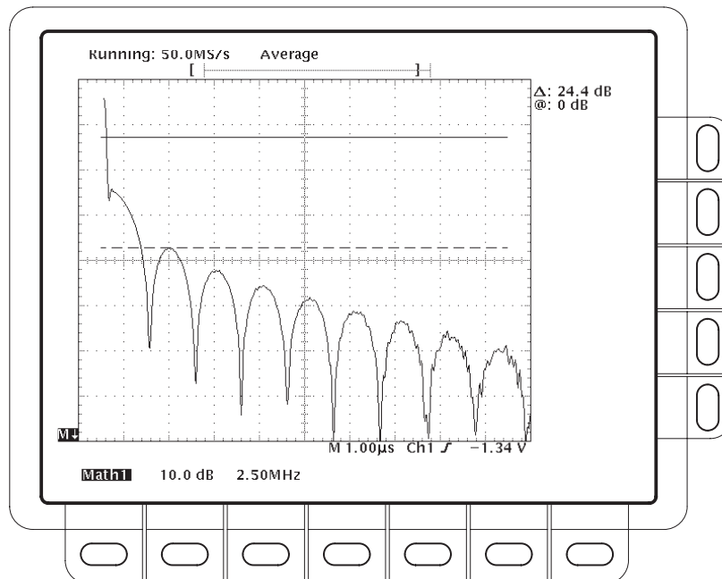
Figure 3-18: Cursor Measurement of an FFT Waveform
