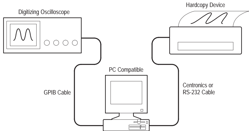
Figure 3-29: Connecting the Digitizing Oscilloscope and Hardcopy Device Via a PC
