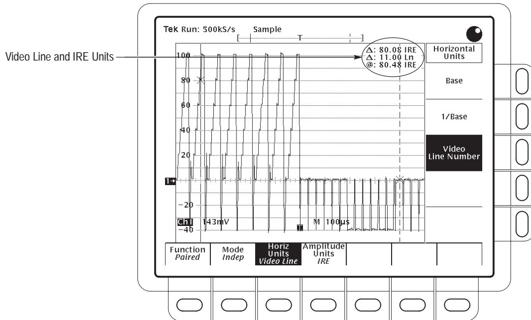
Figure 3-66: Video Line and IRE Units (TDS 400A shown)
