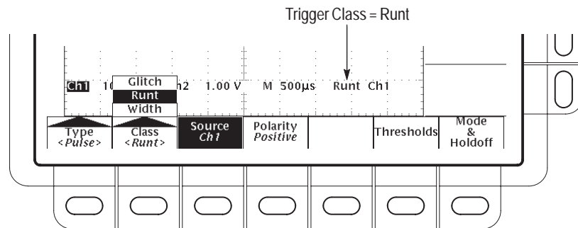
Figure 3-48: Pulse Trigger Readouts
