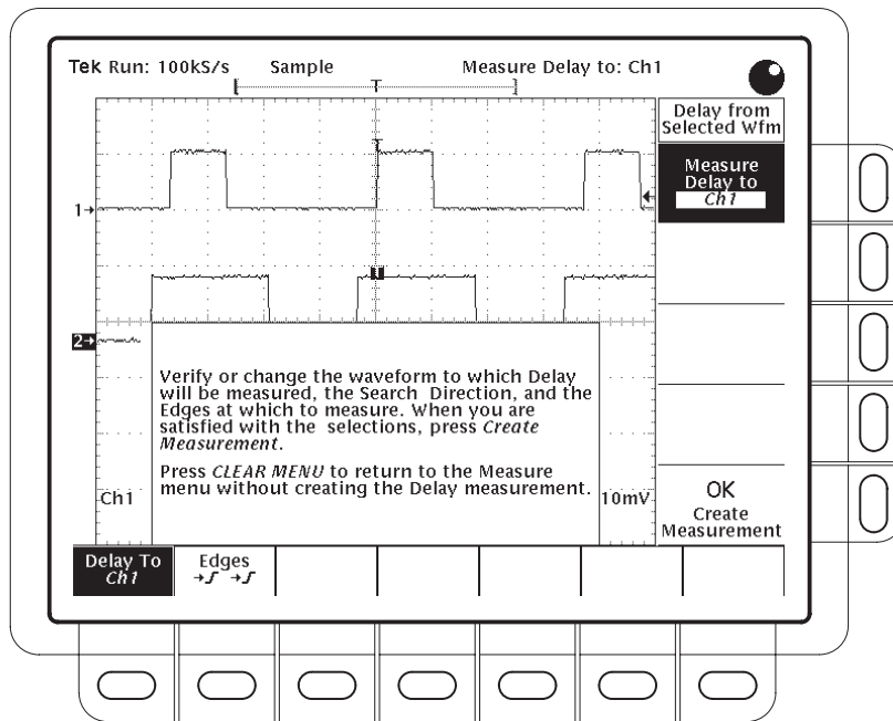
Figure 3-42: Measure Delay Menu — Delay To
