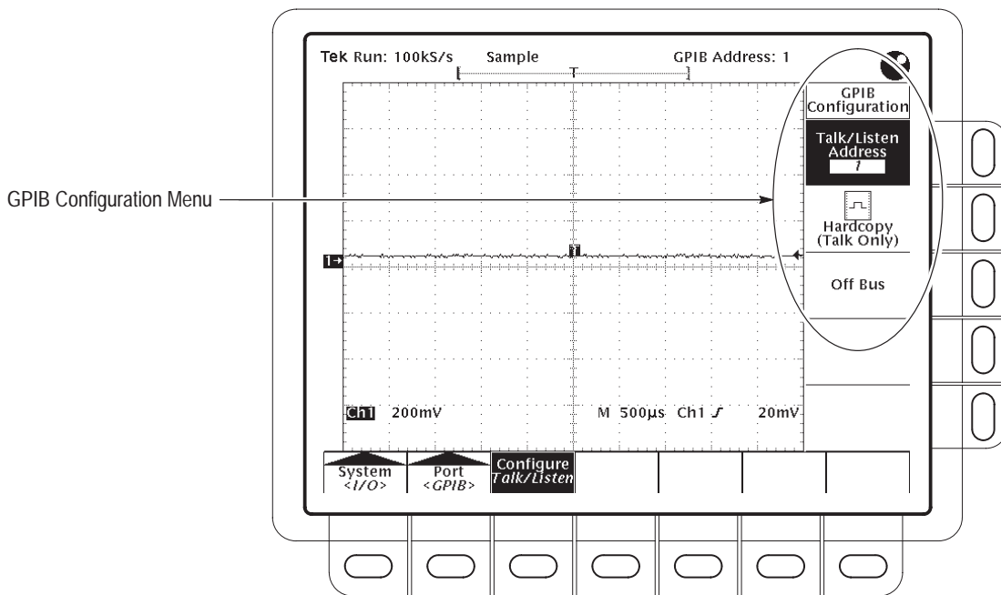
Figure 3-52: Utility Menu
