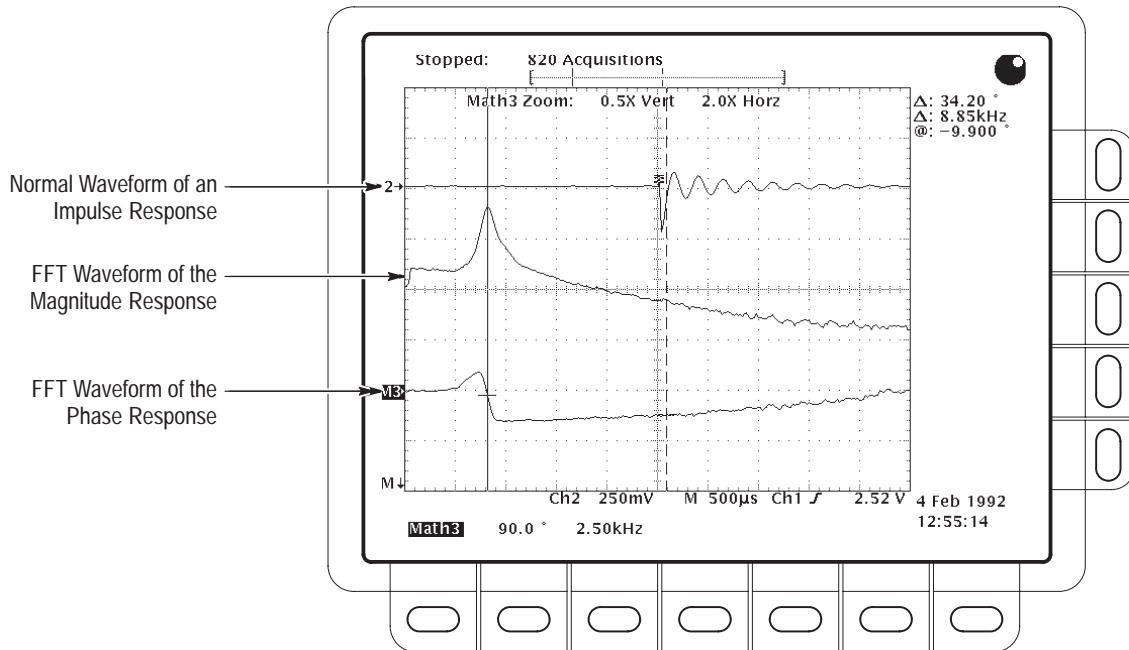
Figure 3-15: System Response to an Impulse
