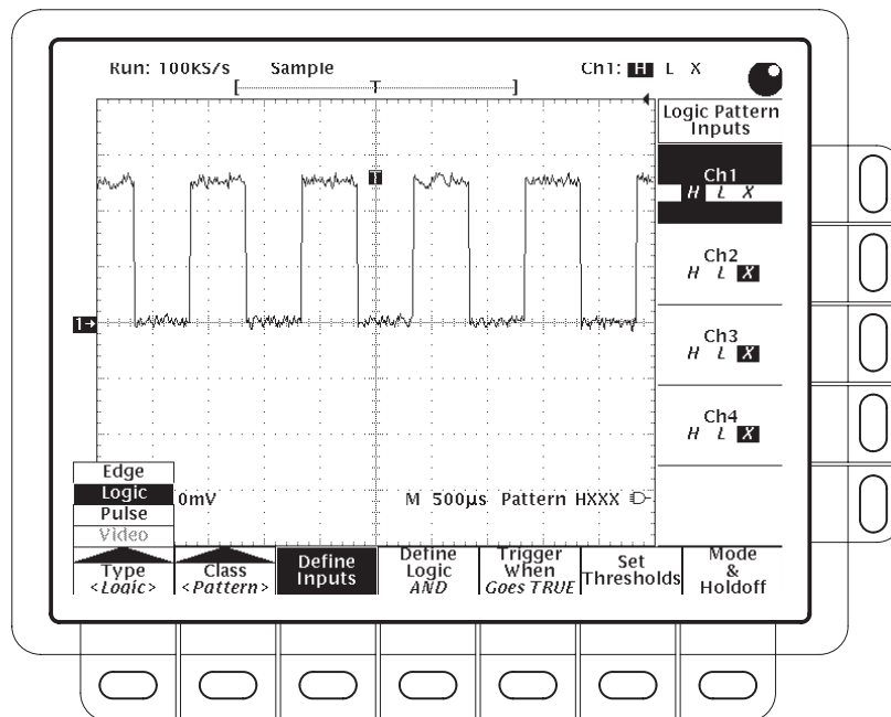
Figure 3-36: Logic Trigger Menu
