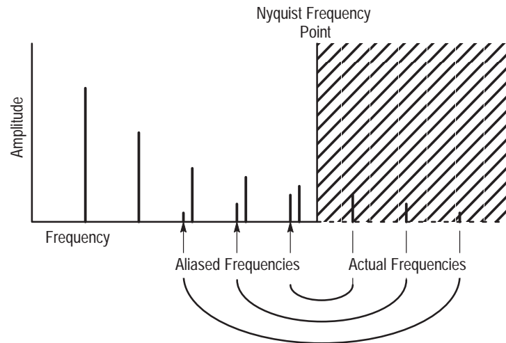
Figure 3-21: How Aliased Frequencies Appear in an FFT
