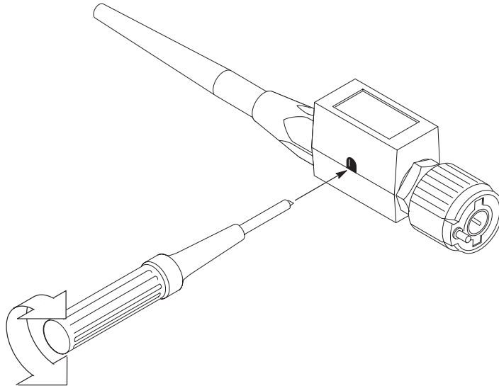
Figure 3-47: Probe Adjustment
