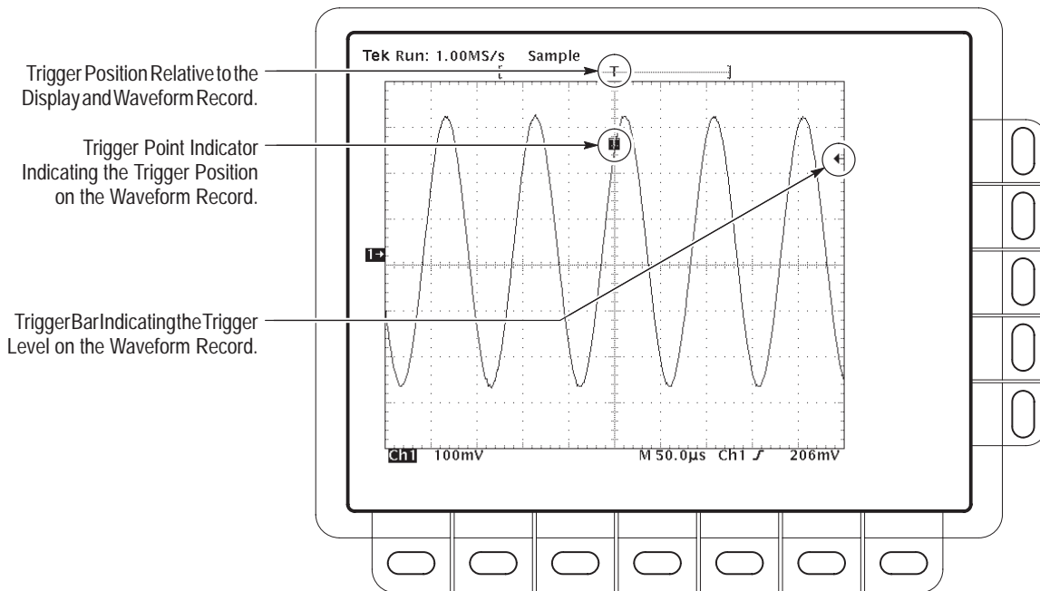
Figure 3-12: Record View, Trigger Position, and Trigger Level Bar Readouts
