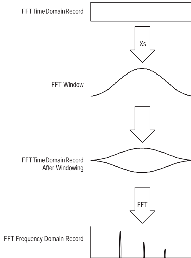
Figure 3-22: Windowing the FFT Time Domain Record
