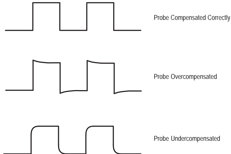
Figure 3-46: How Probe Compensation Affects Signals
