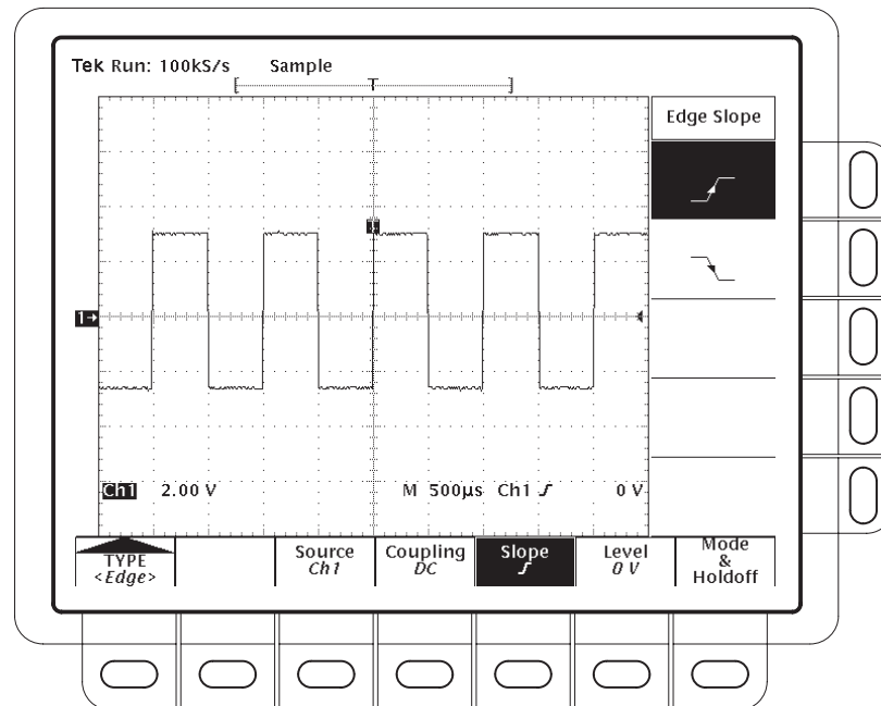
Figure 3-13: Main Trigger Menu — Edge Type
