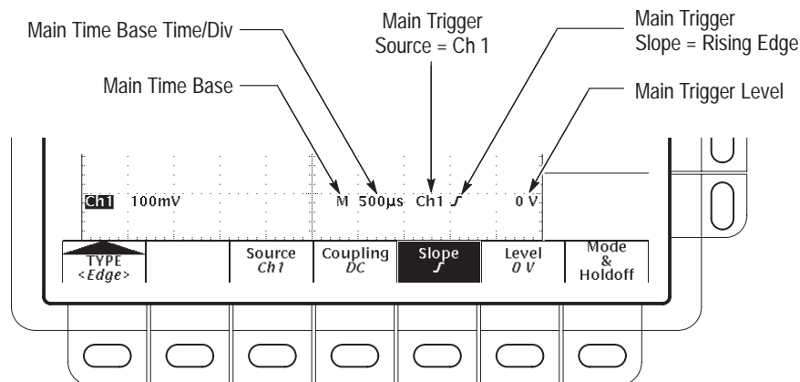
Figure 3-11: Edge Trigger Readouts
